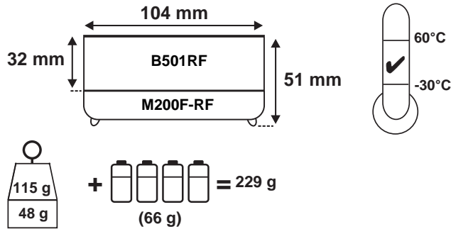
Figure 1: B501RF Mounting
